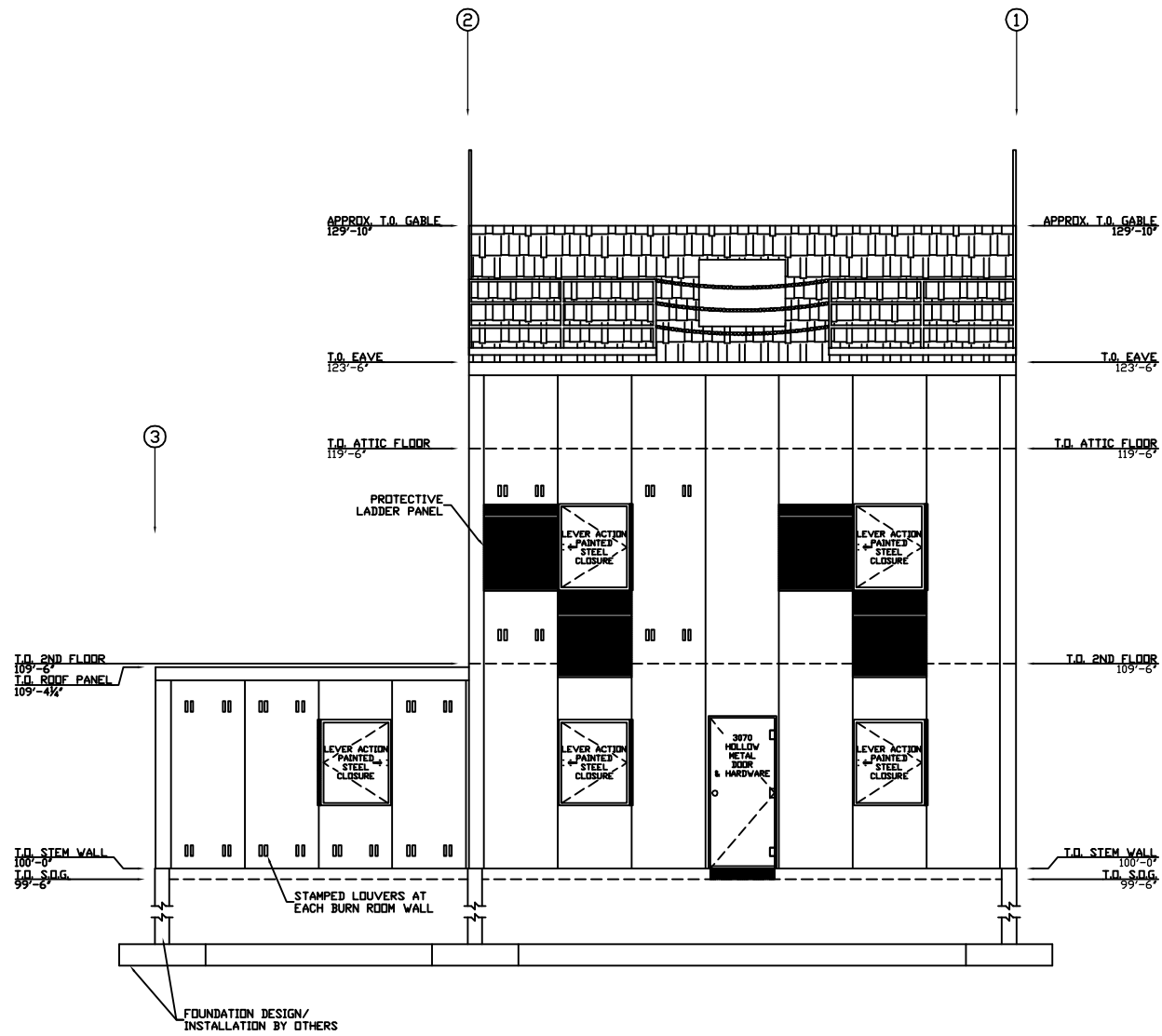
REAR SIDE ELEVATION NOT TO SCALE
