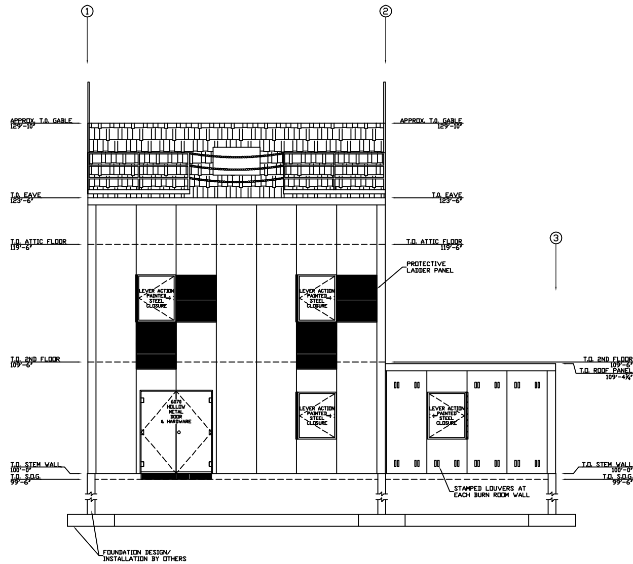
FRONT SIDE ELEVATION NOT TO SCALE
