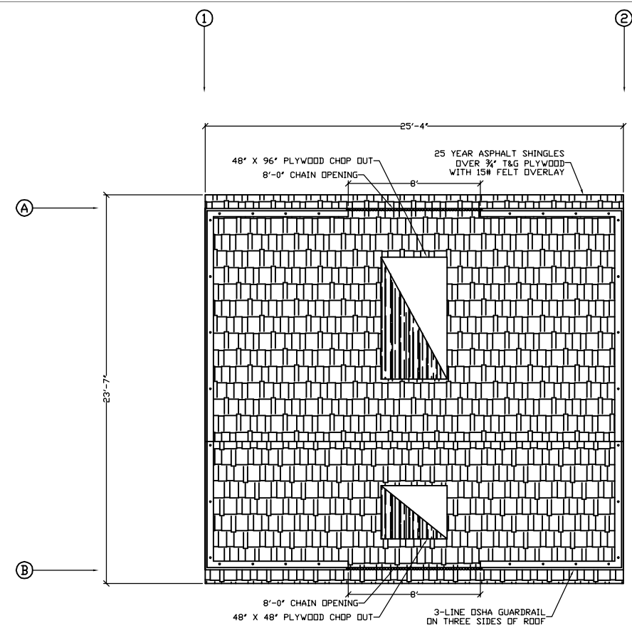
RESIDENTIAL ROOF PLAN NOT TO SCALE
