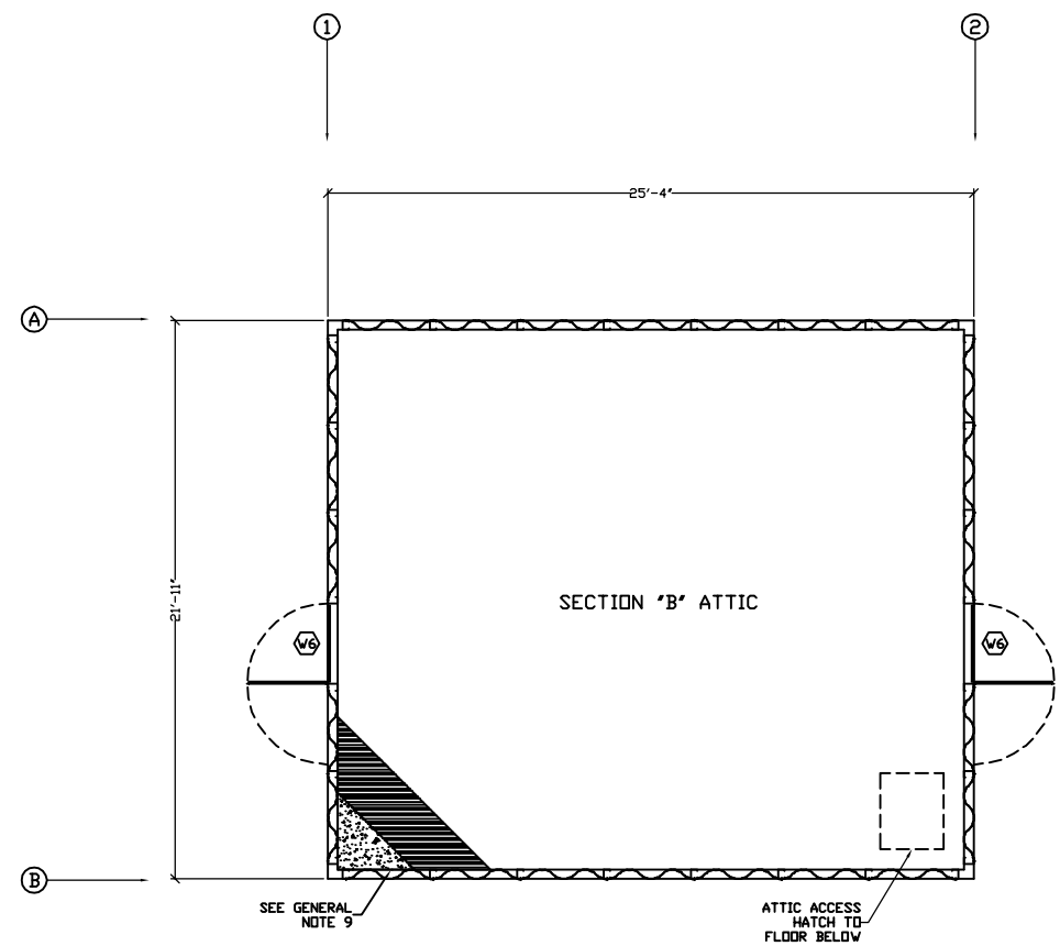
RESIDENTIAL ATTIC PLAN NOT TO SCALE
