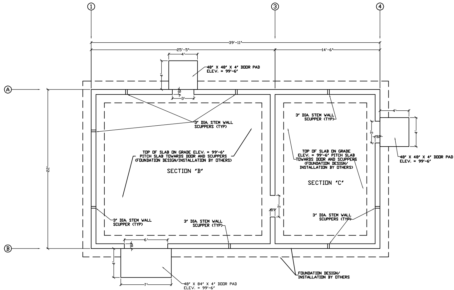
CONCEPTUAL FOUNDATION LAYOUT NOT TO SCALE
