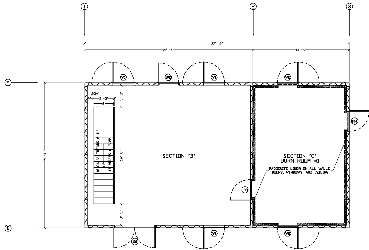
RESIDENTIAL AND ANNEX 1ST FLOOR PLAN NOT TO SCALE
