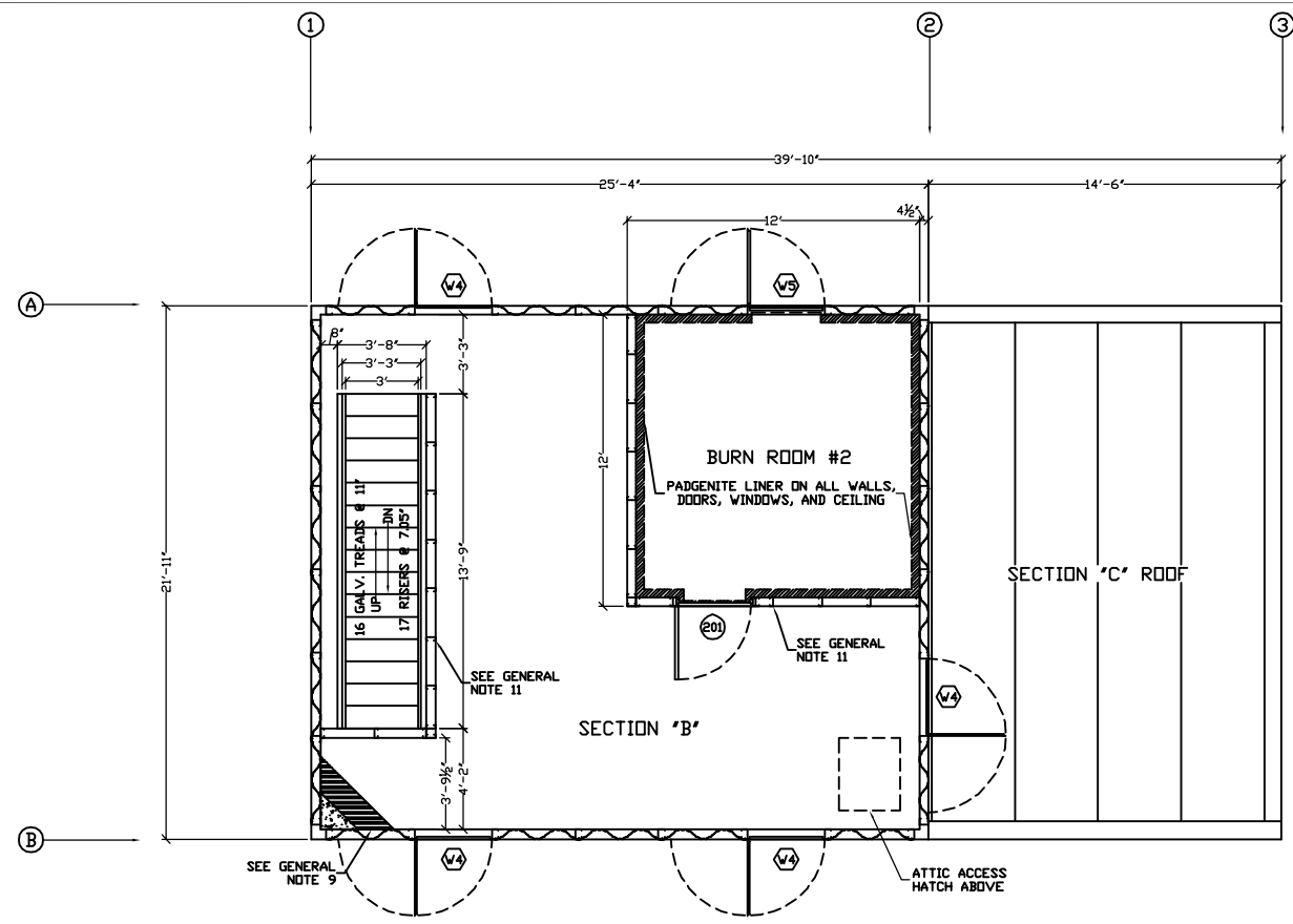
2ND FLOOR PLAN AND ANNEX ROOF PLAN NOT TO SCALE
