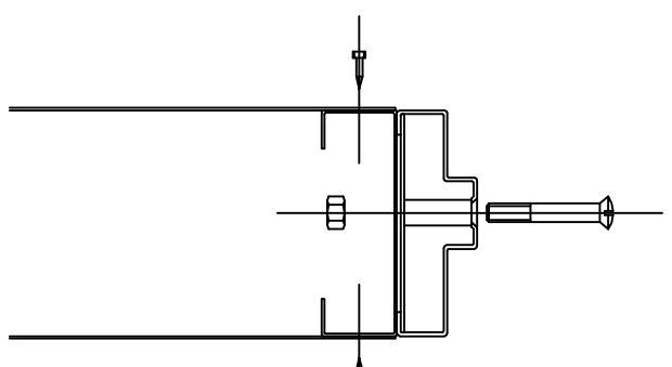
JAMB @ INTERIOR WALL NOT TO SCALE
