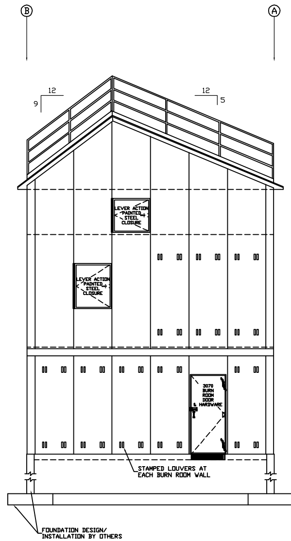
RIGHT SIDE ELEVATION NOT TO SCALE
